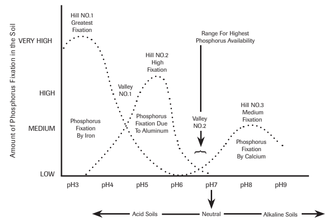
Figure 1. Phosphorus Fixation
